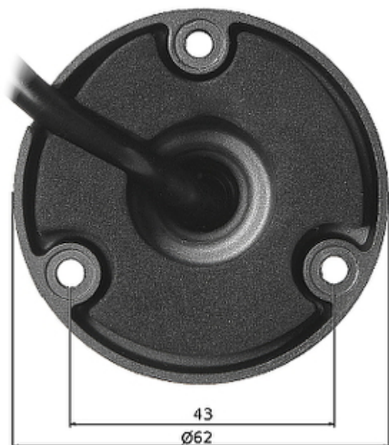
Bracket dimensions:
