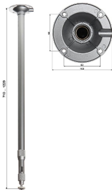
Bracket dimensions:
