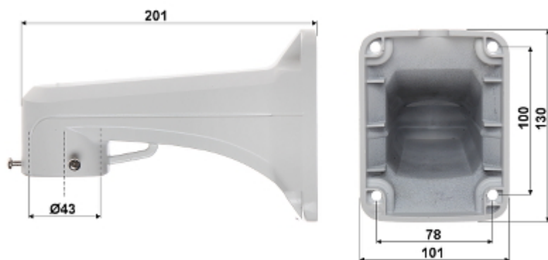
Bracket dimensions:
