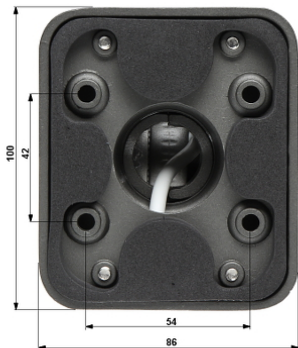
Bracket dimensions:
