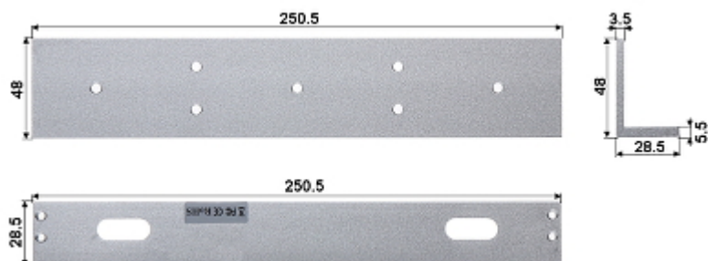
Z-bracket:
