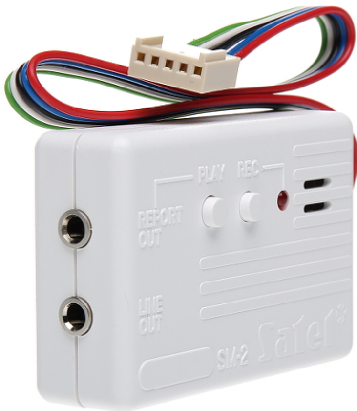
Side view:
