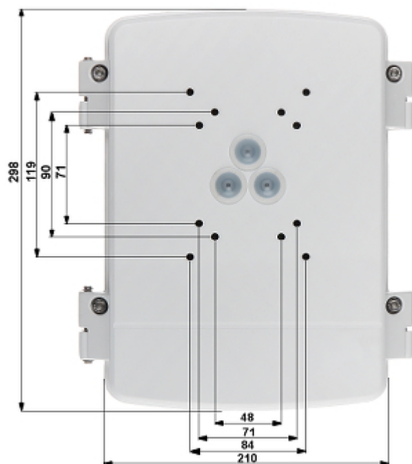
Wall mounting side view:
