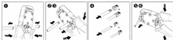
Insulation stripper for cables: UTP, YTKSY
