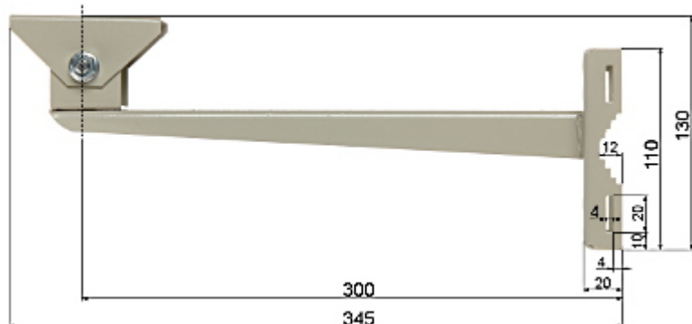
Bracket dimensions:
