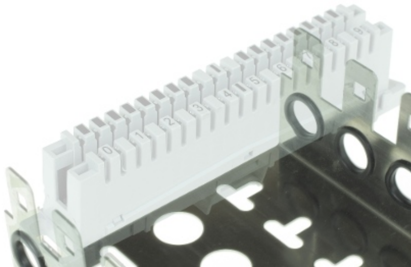
Twisted-pair cable mounting using a KRONE impact tool (ZAC/LSA-P):
