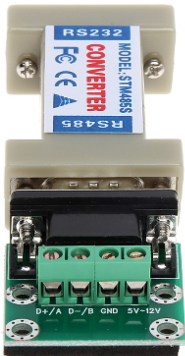
RS-232 connectors:
