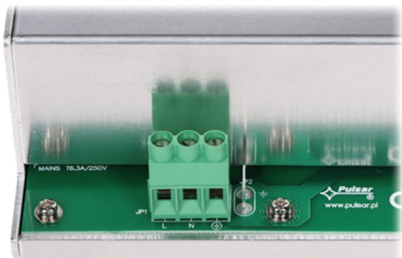
L - Live wire (230V) N - Neutral wire
