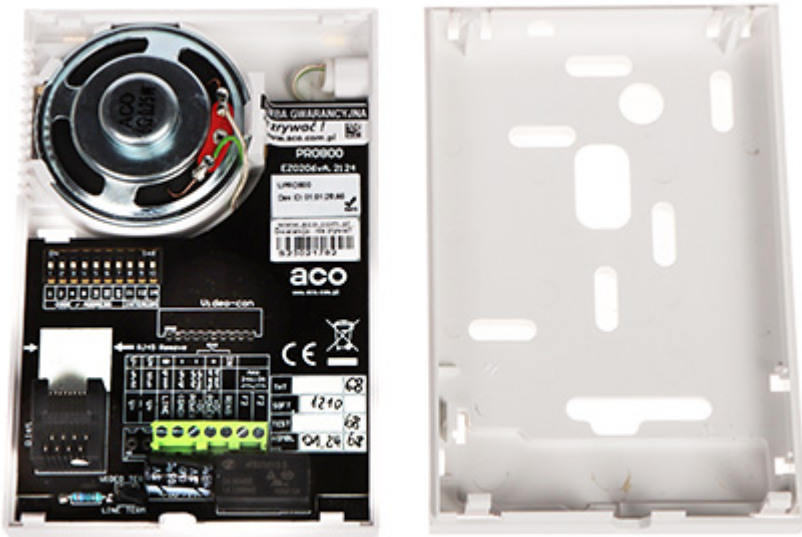
Connectors
