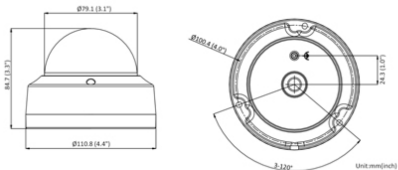
Camera dimensions:
