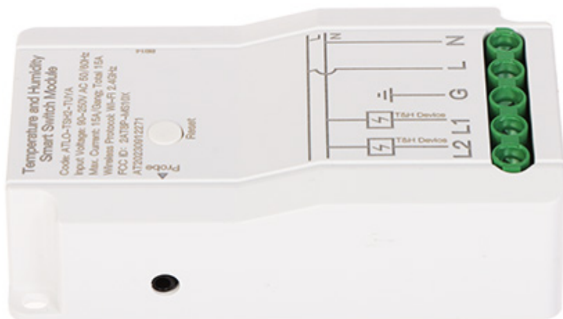
Sensor connector:
