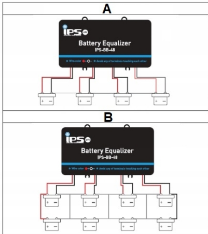
A - 4 batteries in a 48V (4*12V) system B - Multiple sets of batteries
