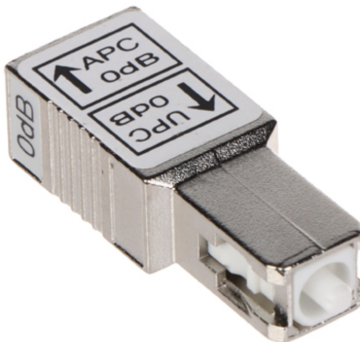
Single-mode adapter connecting SC/APC plug and UPC socket.
