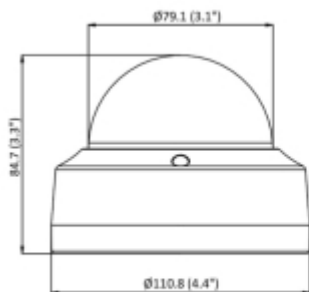
Camera dimensions:
