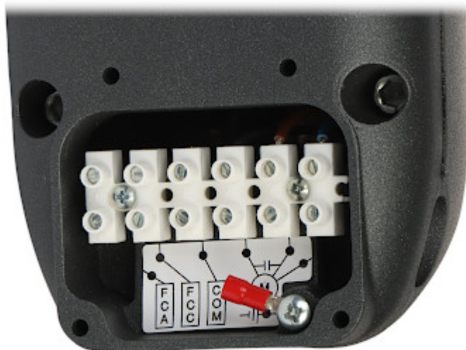
Gate operator controller:
