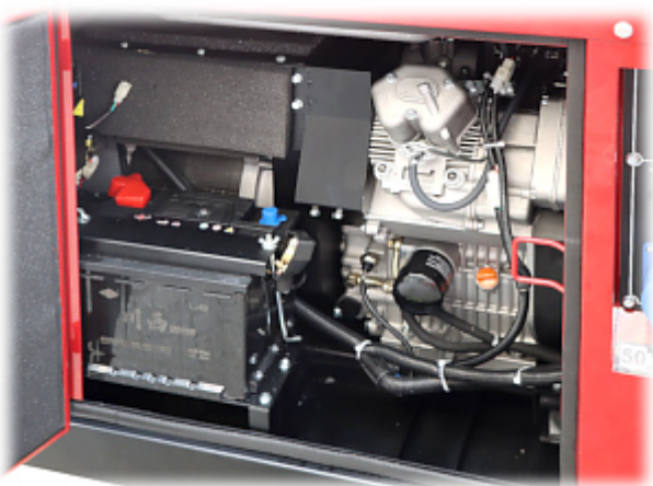
Oil filter and oil filler:
