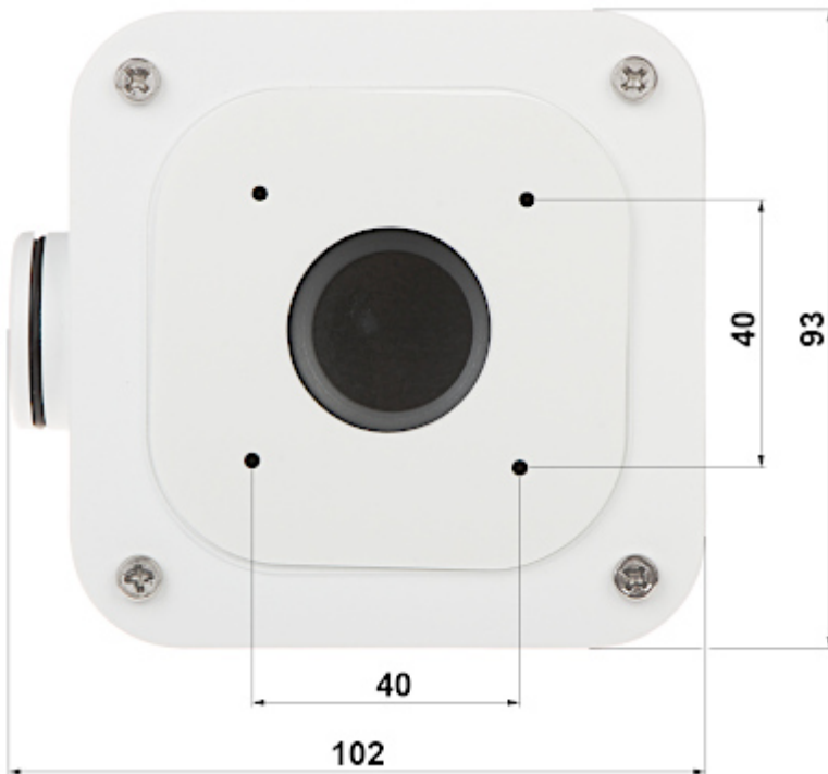
View of the ceiling mounting side
