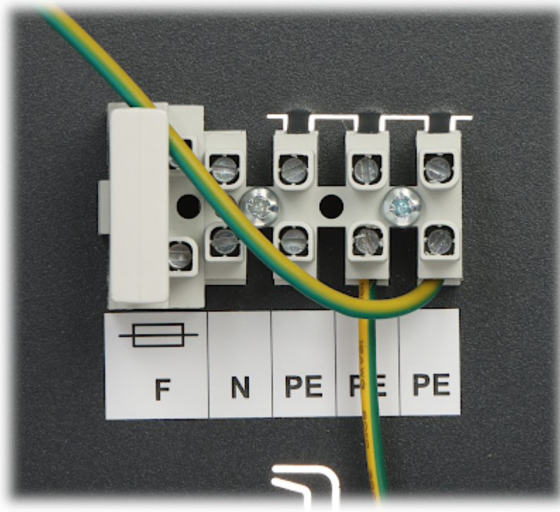
Connectors description:
