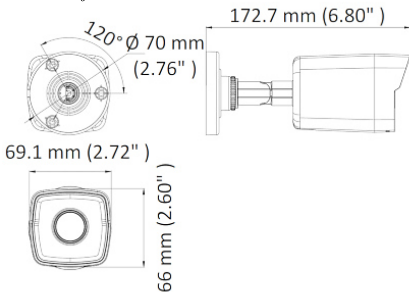
Camera mounting dimensions:
