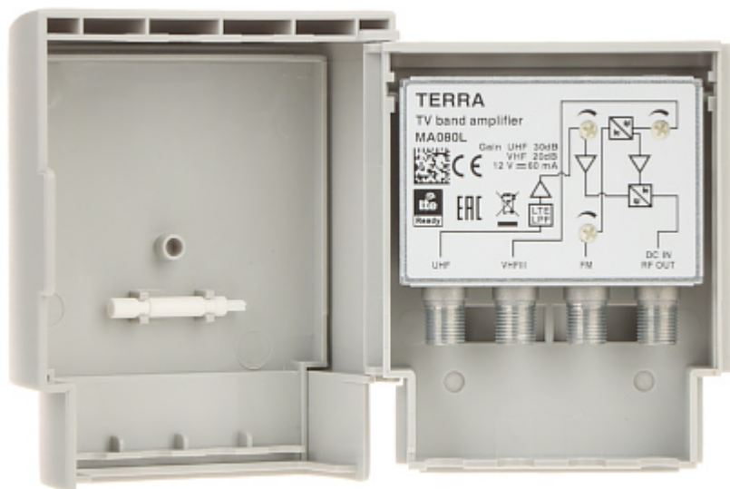
Amplifier with closed enclosure:
