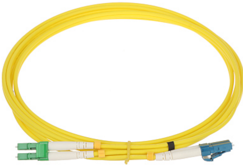
Patchcord connectors
