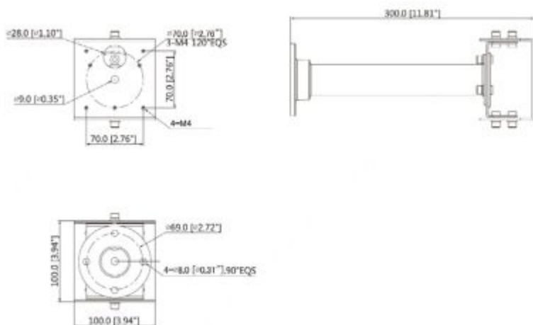
Bracket dimensions:
