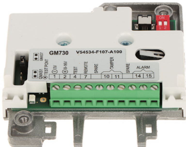
Connectors description:
