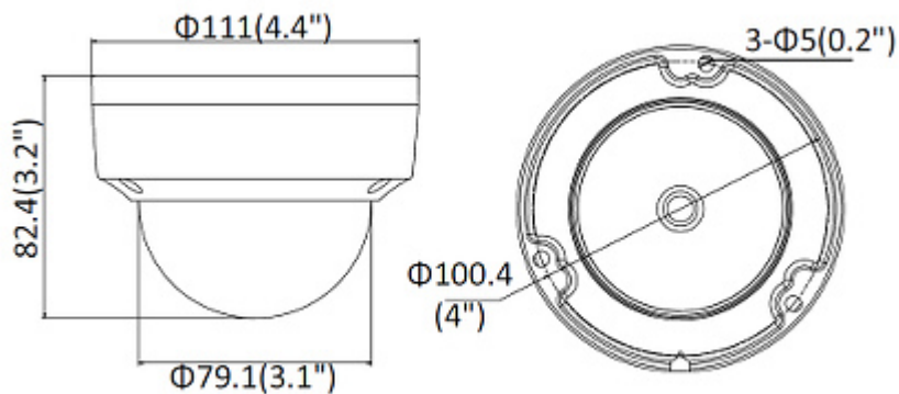
Camera dimensions:
