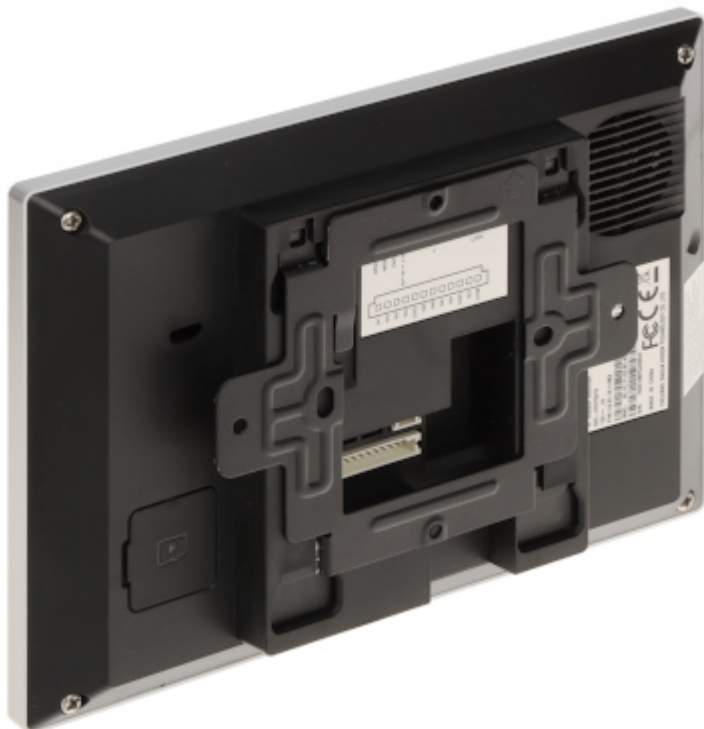
Connectors view:
