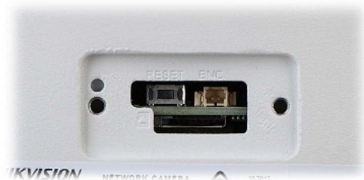
Camera connectors:
