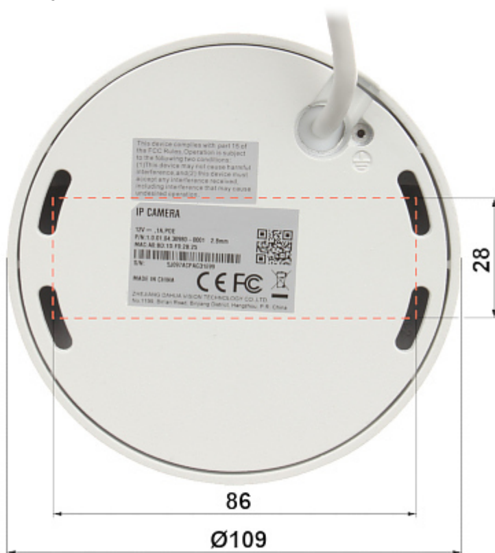
Camera dimensions:
