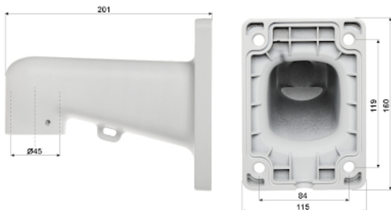
Camera dimensions:
