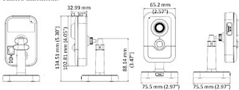
Camera dimensions:
