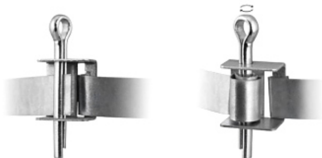
The correct mounting of the strip:
