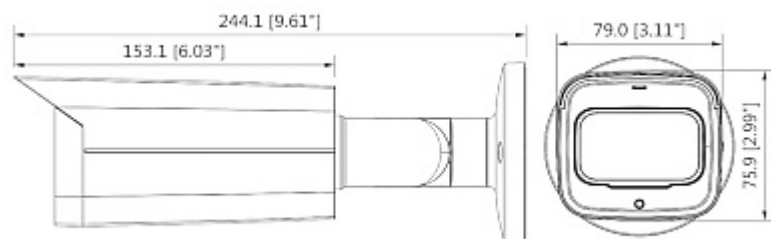
Camera dimensions:
