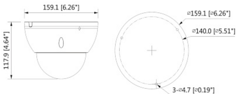
Camera dimensions:
