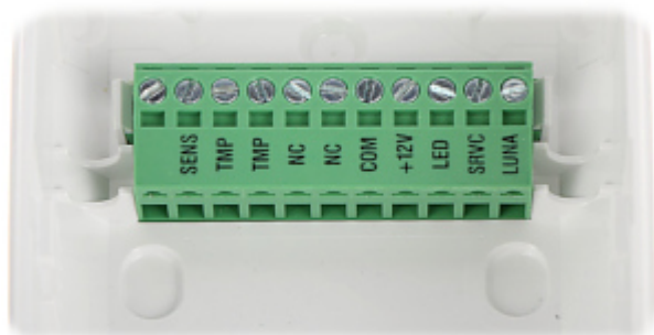
Rear view:
