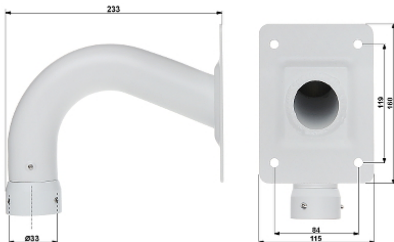
Camera dimensions:
