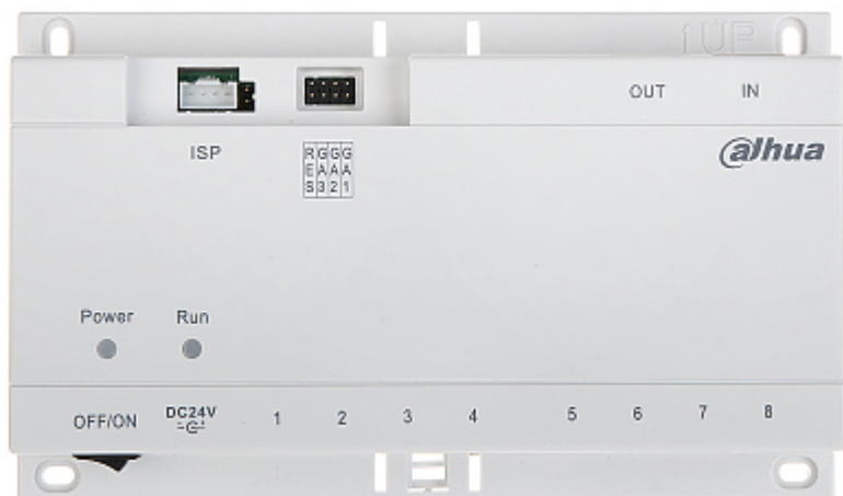
Connectors view:
