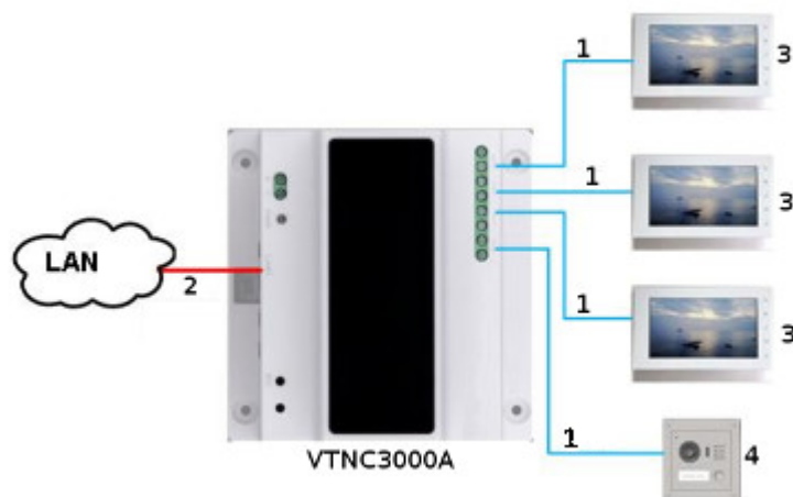
Connection schematic diagram:
