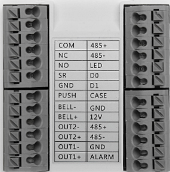
Device connectors:
