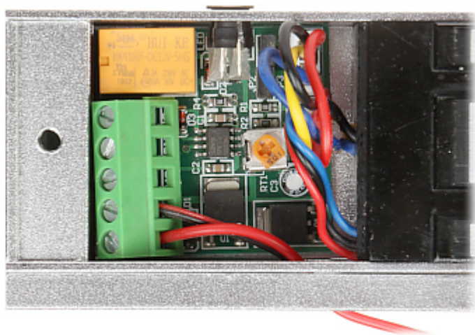
Internal view:
