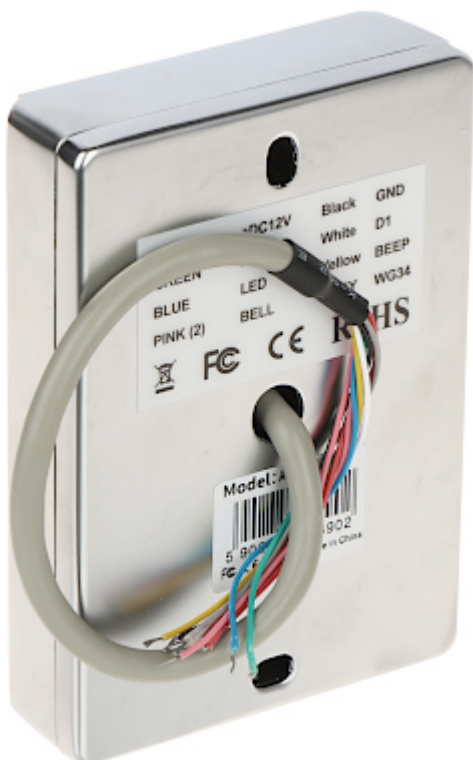
Connectors description:
