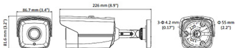
Mounting side view:
