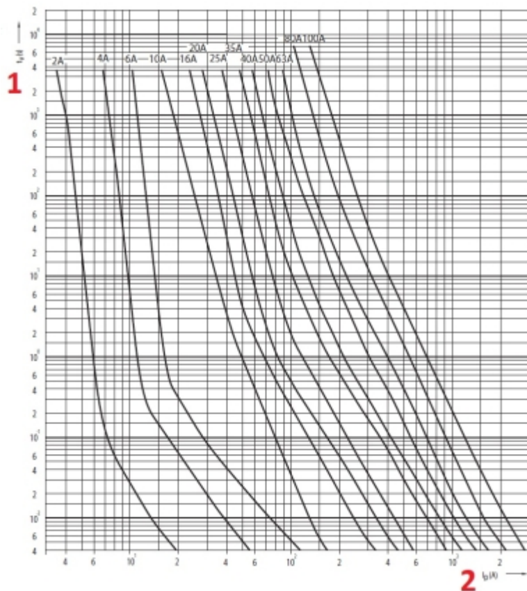
Time-current characteristics:
