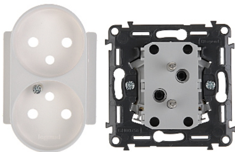
Rear view:
