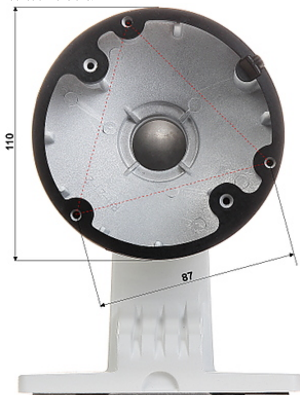
Bracket dimensions:
