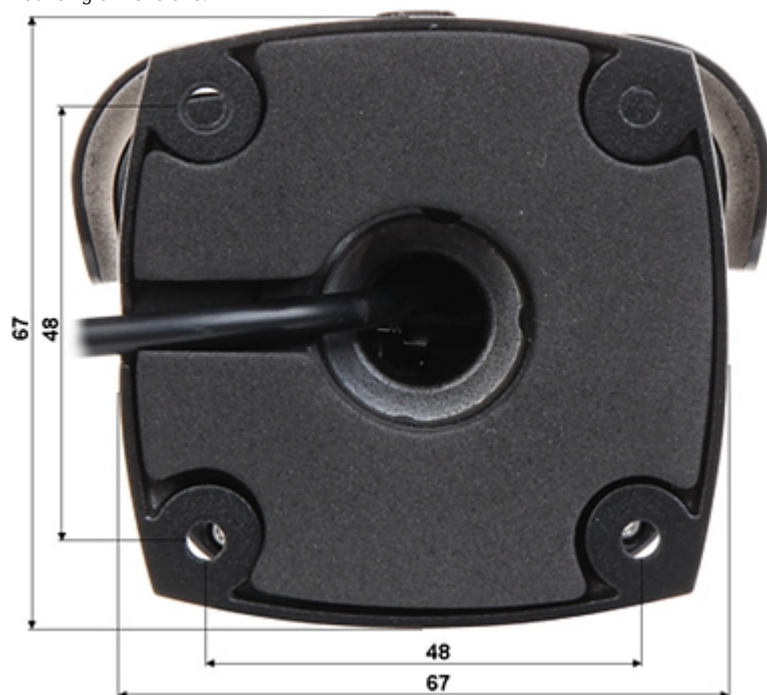
Mounting dimensions:
