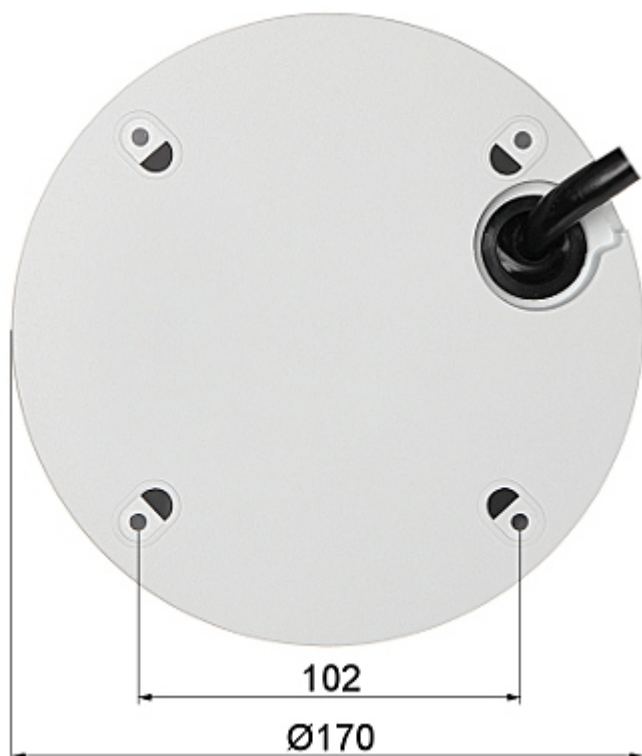
Camera dimensions:
