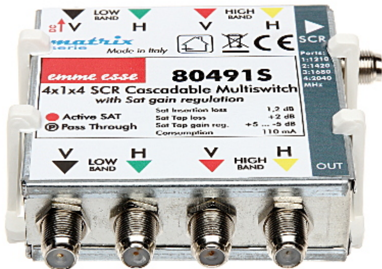
Connectors view:
